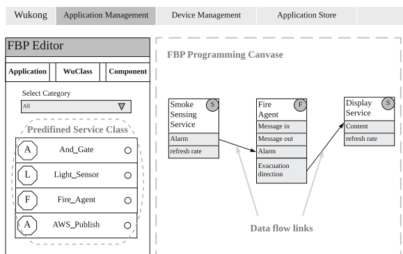
Fig. 5. Example application in the WuKong FBP environment.
