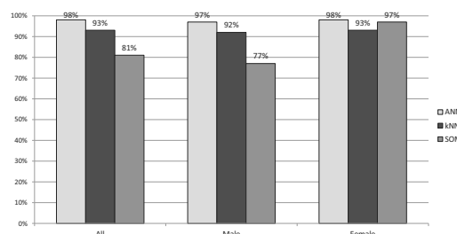
Fig. 9. Comparison of accuracy results for various automatic classification methods using the Time+SPEC+modMFCC vector of features.
