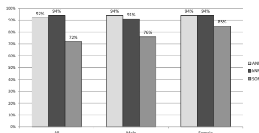
Fig. 8. Comparison of accuracy results for various automatic classification methods using the Time+SPEC vector of features.
