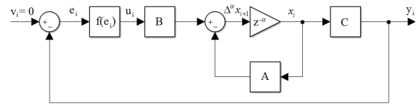
Fig. 3. Fractional nonlinear discrete-time system.
