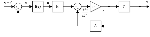
Fig. 1. Fractional nonlinear continuous-time system.
