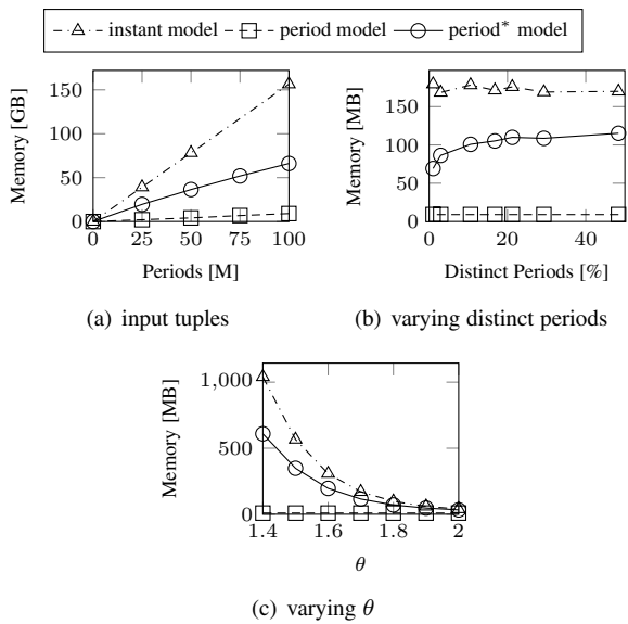
Fig. 12. Storage costs for the dataset SYNTH.
