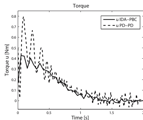
Fig. 6. Input control supplied from the IDA-PBC (76) in comparison with the torque of the cascade PD-PD controller (90).
