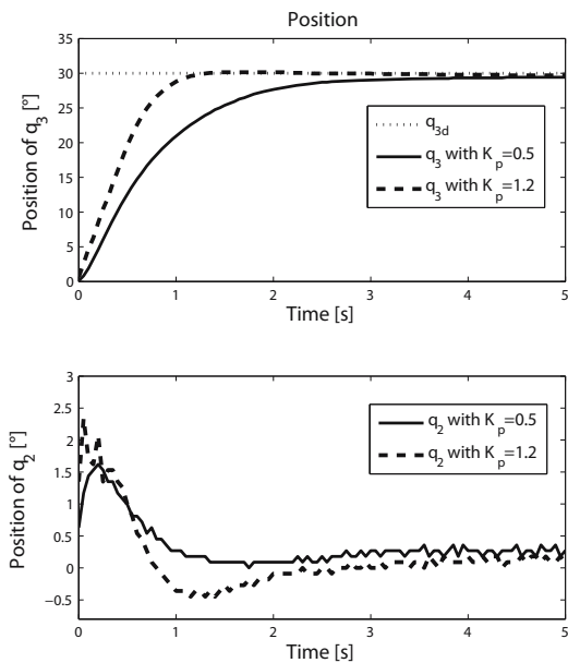
Fig. 8. Time evolution of q_3 and q_2 utilizing the IDA-PBC (76) for different values of K_p .
