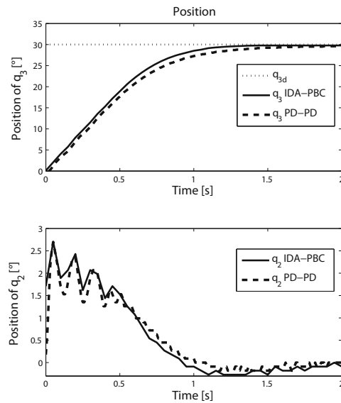
Fig. 5. Time evolution of q_3 and q_2 utilizing the IDA-PBC (76) in comparison with the cascade PD-PD controller (90).
