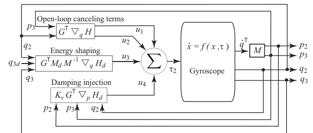
Fig. 3. Block diagram of the IDA-PBC (76) applied to a 2-DOF gyroscope.
