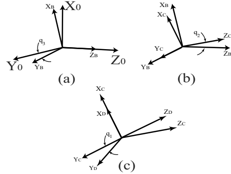
Fig. A2. Relative movement of each frame of the gyroscope.
