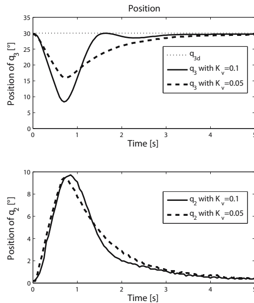
Fig. 9. Time evolution of q_3 and q_2 utilizing the IDA-PBC (76) rejecting disturbances with different values of K_v .
