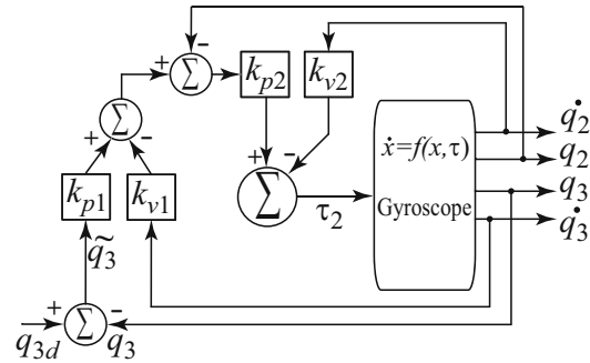
Fig. 4. Block diagram of the cascade PD-PD controller (90) applied to the gyroscope to compare it with the IDA-PBC (76).
