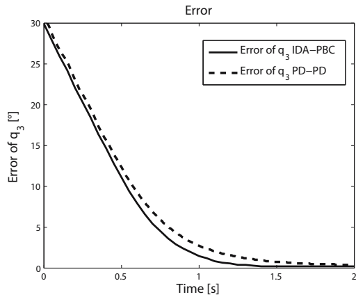
Fig. 7. Position error, \tilde{q}_3 = q_{3d} - q_3 utilizing the IDA-PBC (76) and the cascade PD-PD controller (90).
