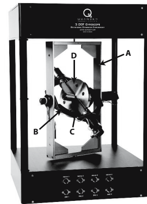
Fig. 1. Gyroscope by Quanser and the body nomenclature.
