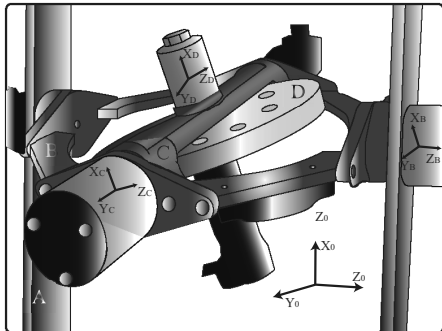
Fig. A1. Schematic representation of the gyroscope in an arbitrary configuration.
