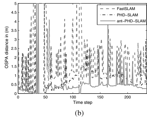
Fig. 9. OSPA distance of map features by different approaches: Case 1 (a), Case 2 (b).
