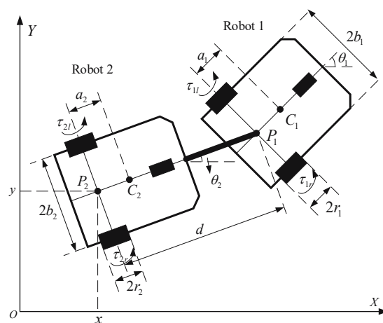
Fig. 1. Two differential 2WD robots with a physical link.
