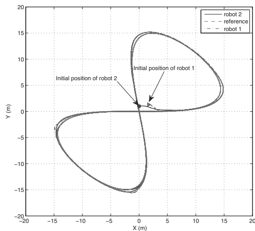
Fig. 4. Robot trajectories in the (x, y) plane.
