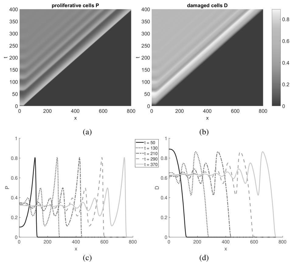
Fig. 4. Solutions of system (3) with the initial condition P(0, x) = 0.05 for x \leq 30 and 0 otherwise, while D(0, x) = 0 for all x , x \in [0, 800] , t \in [0, 400] . Parameters: \beta = 0.05 , k = 2 . Panel (a): propagation of variable P in (x, t) space, panel (b): propagation of variable D in (x, t) space, panel (c): selected profiles for variable P , panel (d): selected profiles for variable D (selected times as in panel (c)). The wave moves right with a numerically calculated speed 1.97.
