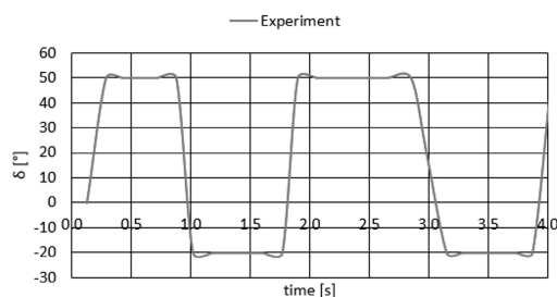
Fig. 14. Fin deflection angle for a diving test (input).
