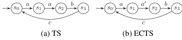
Fig. 4. TS before label splitting (a) and ECTS after label splitting (b).
