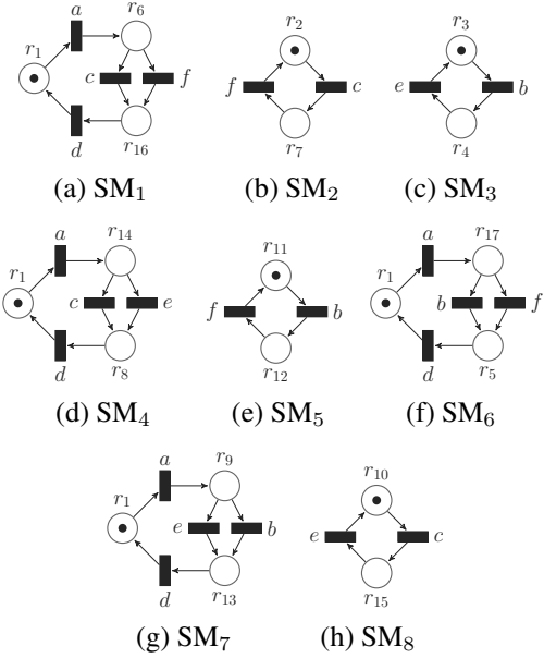
Fig. 5. All SMs created from the TS in Fig. 3.
