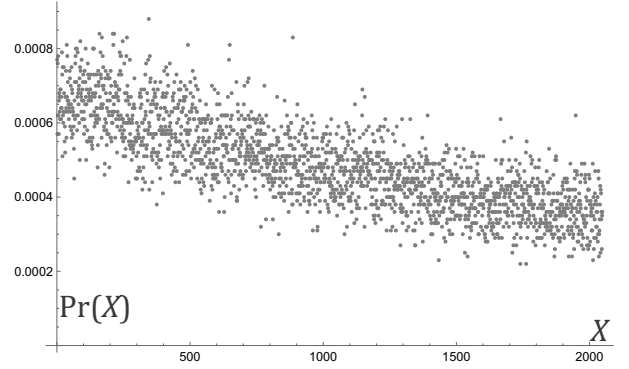
Fig. 6. Example of probability distribution of X = x - L for L = 2048 and m = 256 and a fast symbol spread.
