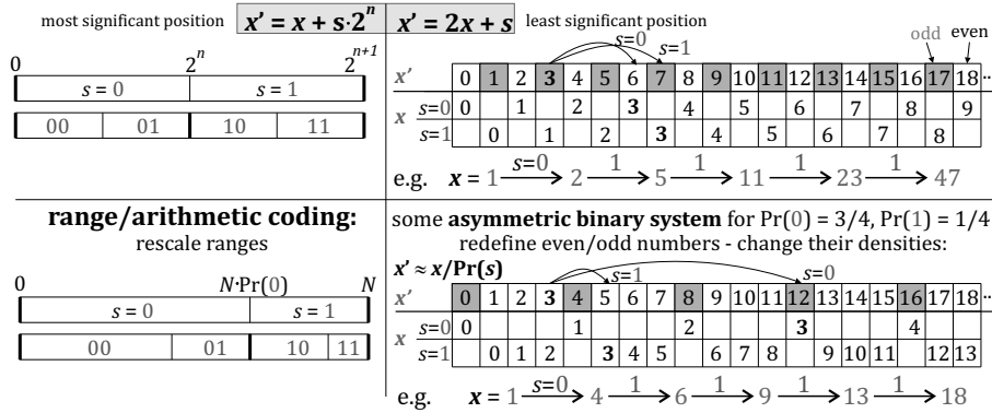
Fig. 2. Arithmetic coding (left) and ANS (right) seen as an asymmetrization of the standard numeral system—in order to optimize them for storing symbols from a general probability distribution.
