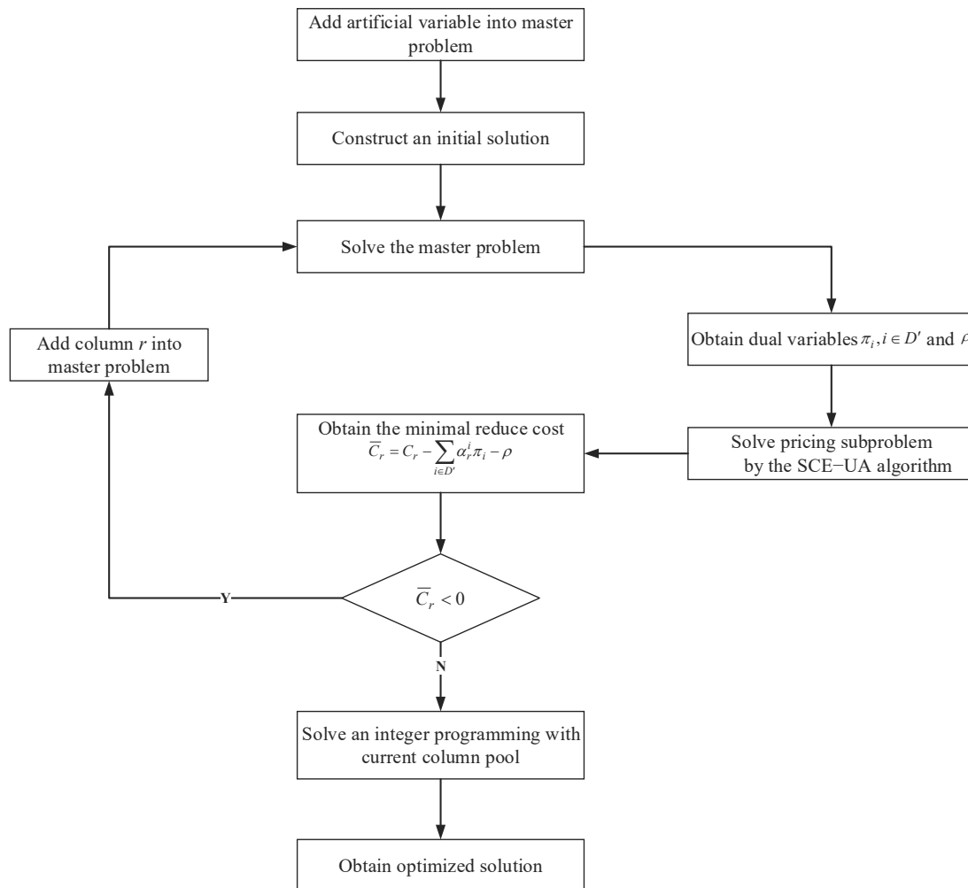
Fig. 2. Framework of column generation.
