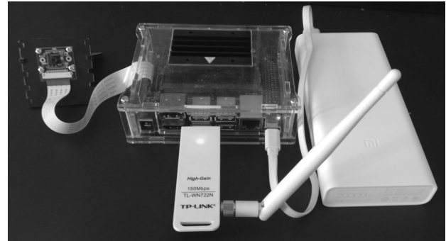
Fig. 2. IoT monitoring device used for bee observation and varroosis detection.
