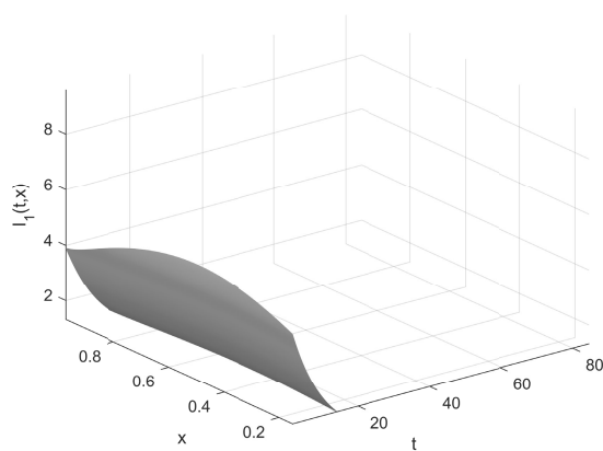
(a) state trajectories for I_1(t, x)
