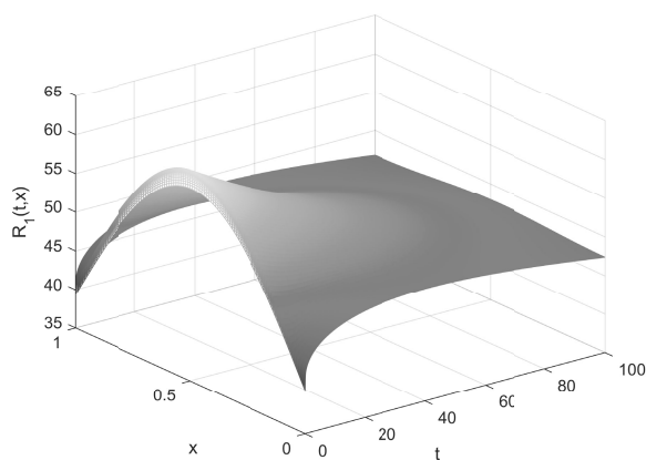
(a) state trajectories for R_1(t, x)
