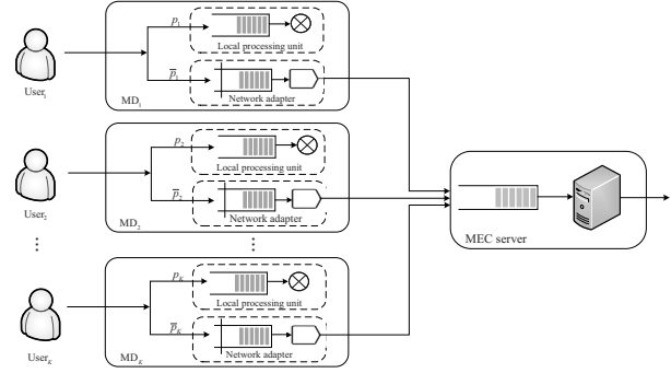
Fig. 1. Architecture of the MEC system.
