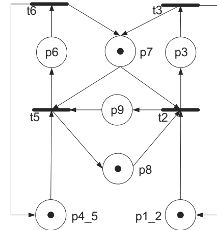
Fig. 3. Reduced Petri net.
