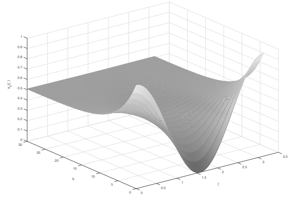
Fig. 1. Plant state trajectory (x_k(\xi))_{k=0}^{30} .
