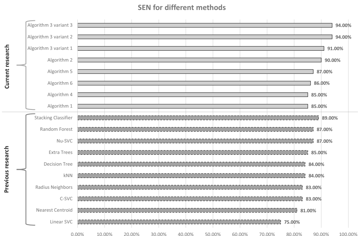
Fig. 18. SEN for different methods.
