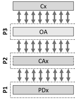
Fig. 2. Pay&amp;Require layer model.
