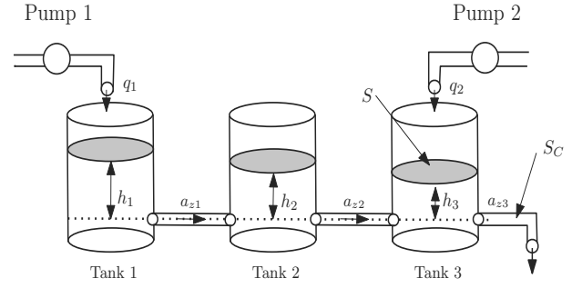
Fig. 2. Structure of the three-tank system.
