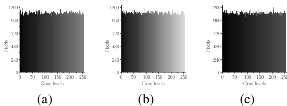
Fig. 4. Basic color distribution of Lena encrypted with the l value for the red (a), green (b) and blue (c) colors.
