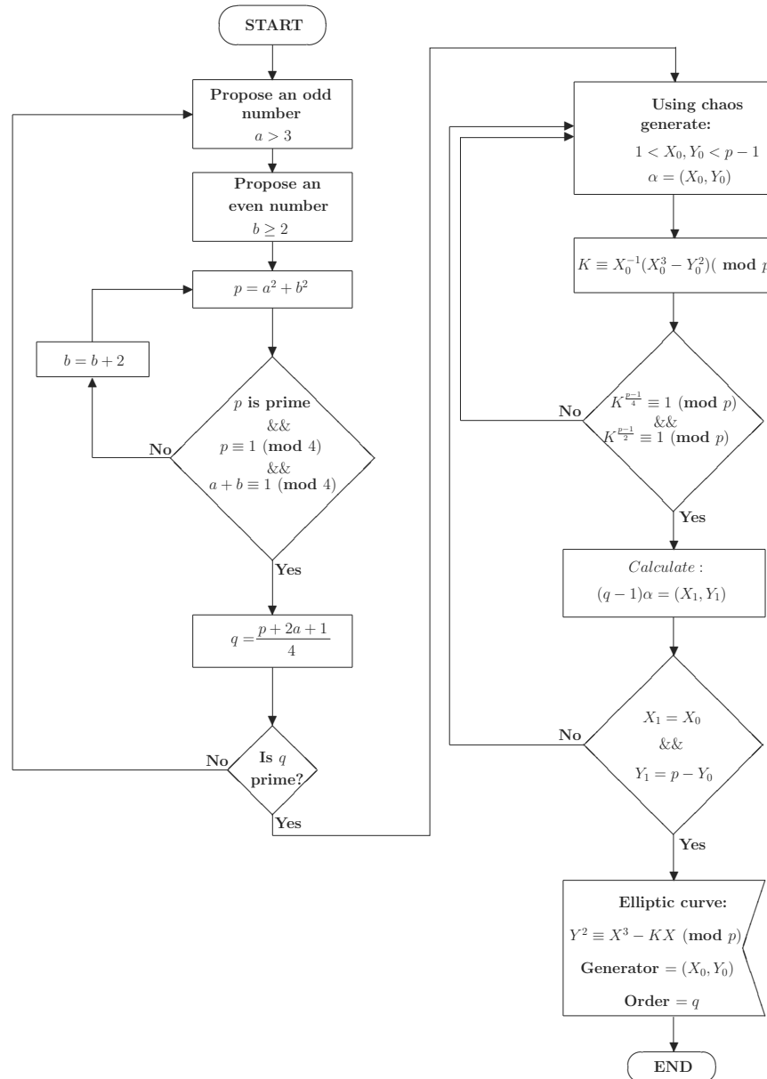
Fig. 1. Elliptic curve flowchart.
