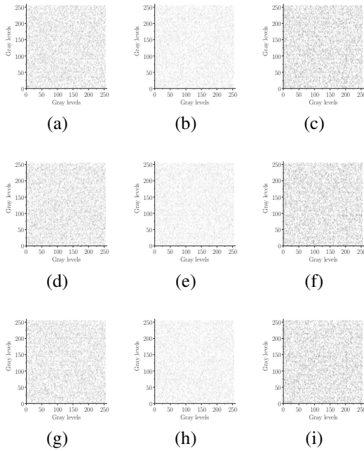
Fig. 3. Points (x_{c,d}, y_{c,d}) for the horizontal direction for the red (a), green (b) and blue (c) colors, for vertical direction (d), (e) and (f), and diagonal direction (g), (h) and (i), using the Lena test image encrypted with the l value.
