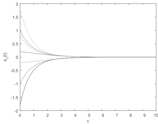
Fig. 1. State x_1(t) of the ISDNN (33) without external disturbances and impulses.
