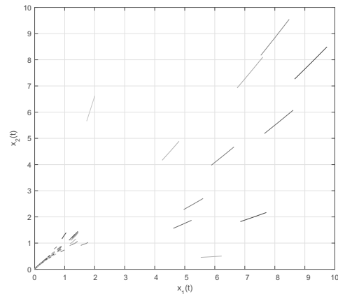
Fig. 9. Phase curves of the system ISDNN (33) quantized by external disturbances and impulses at different initial values.
