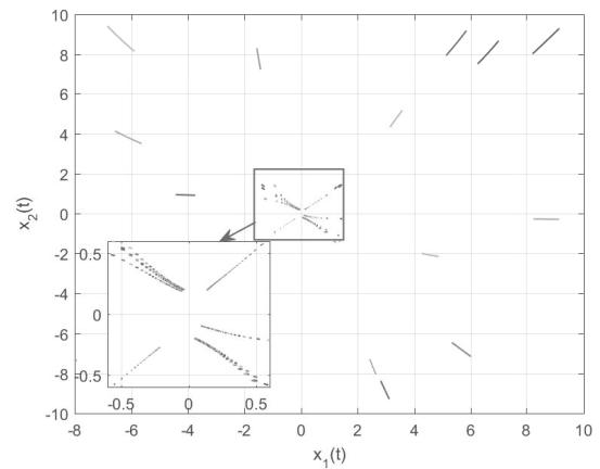
Fig. 4. Phase curves of the ISDNN (33) with nonlinear external disturbances and generated impulsive switching at t = 0.1k, k \in \mathcal{N} , under different initial values.
