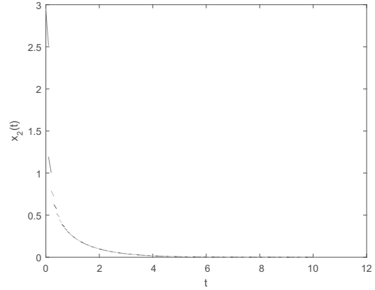
Fig. 8. State x_2(t) of the system ISDNN (33) quantized by external disturbances and impulses.
