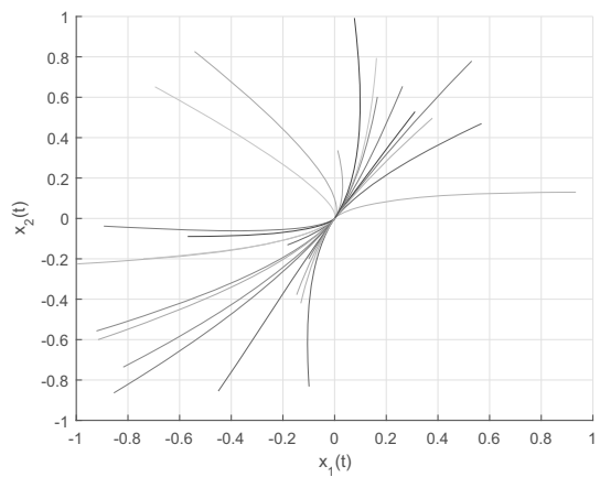
Fig. 3. Phase curves of the SDNN (33) without external disturbances and impulses at different initial values.
