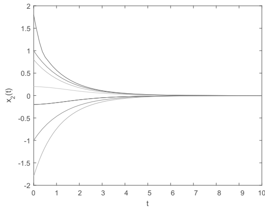
Fig. 2. State x_2(t) of the ISDNN (33) without external disturbances and impulses.
