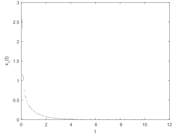
Fig. 7. State x_1(t) of the system ISDNN (33) quantized by external disturbances and impulses.
