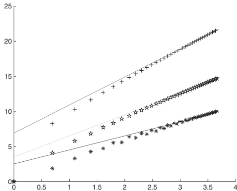
Fig. 1. Fully discretised continuous collocation methods with c = [0, .35, .8, .95] in Example 1. The plotted function is \log(\|e(h)\|) with respect to \log(h) . The symbols (plus, pentagon and star) are used to show the first, the second and the third components of the error function. The lines have respectively the slopes 4, 3 and 2.
