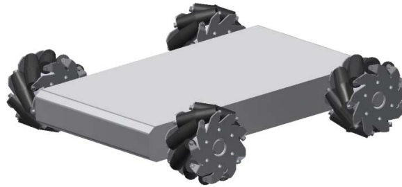
Fig.2. Virtual model of a WMR with mecanum wheels.
