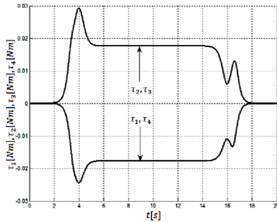
Fig.13. Behaviours of driving moments of wheels no. 1, 2, 3, 4.
