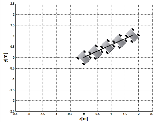
Fig.8. Trajectory of motion of the characteristic point with graphical reflection of configuration of the WMR platform in the course of simulation.
