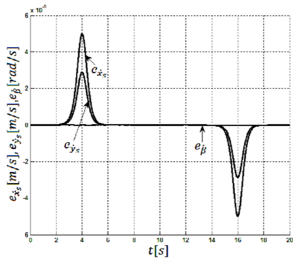
Fig.17. Calculation errors of the projections of velocity of the characteristic point of the WMR: e_{\dot{x}_s}(t), e_{\dot{y}_s}(t) and the angular speed of the frame e_{\dot{\beta}}(t) .
