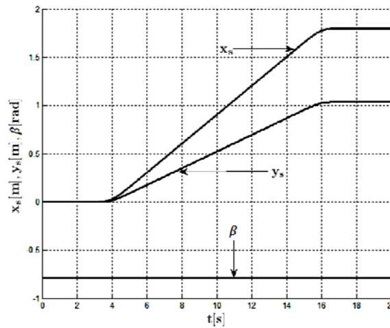
Fig.14. Solution of a forward dynamics problem: behaviours: x_s(t), y_s(t) and \beta(t) .
