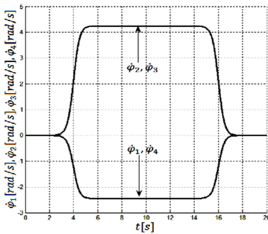
Fig.11. Behaviours of angular velocities of wheels no. 1, 2, 3, 4
