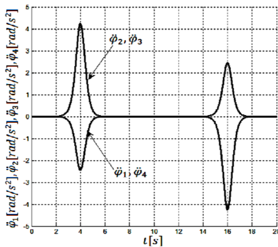
Fig.12. Behaviours of angular accelerations of wheels no. 1, 2, 3, 4.
